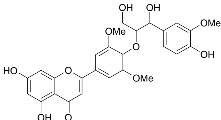
Figure 6: tricin derivatives isolated from Avena sativa herb.
