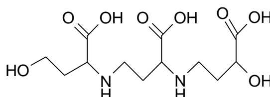
Figure 6: Avenic acid B
