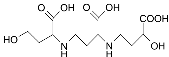
Figure 4: Avenic acid A
