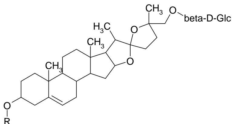
Figure 5: Avenacoside A and Avenacoside B.
